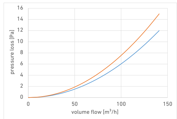
Pressure loss
